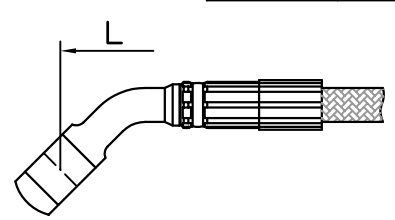
Ringfitting, 45° Alu
